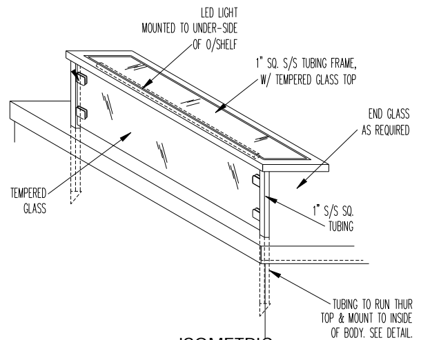
ISOMETRIC 90 SERIES SINGLE TIER WITH GLASS TOP SHELF
